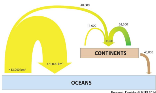
FIGURE 1 Global Terrestrial Water Cycle
